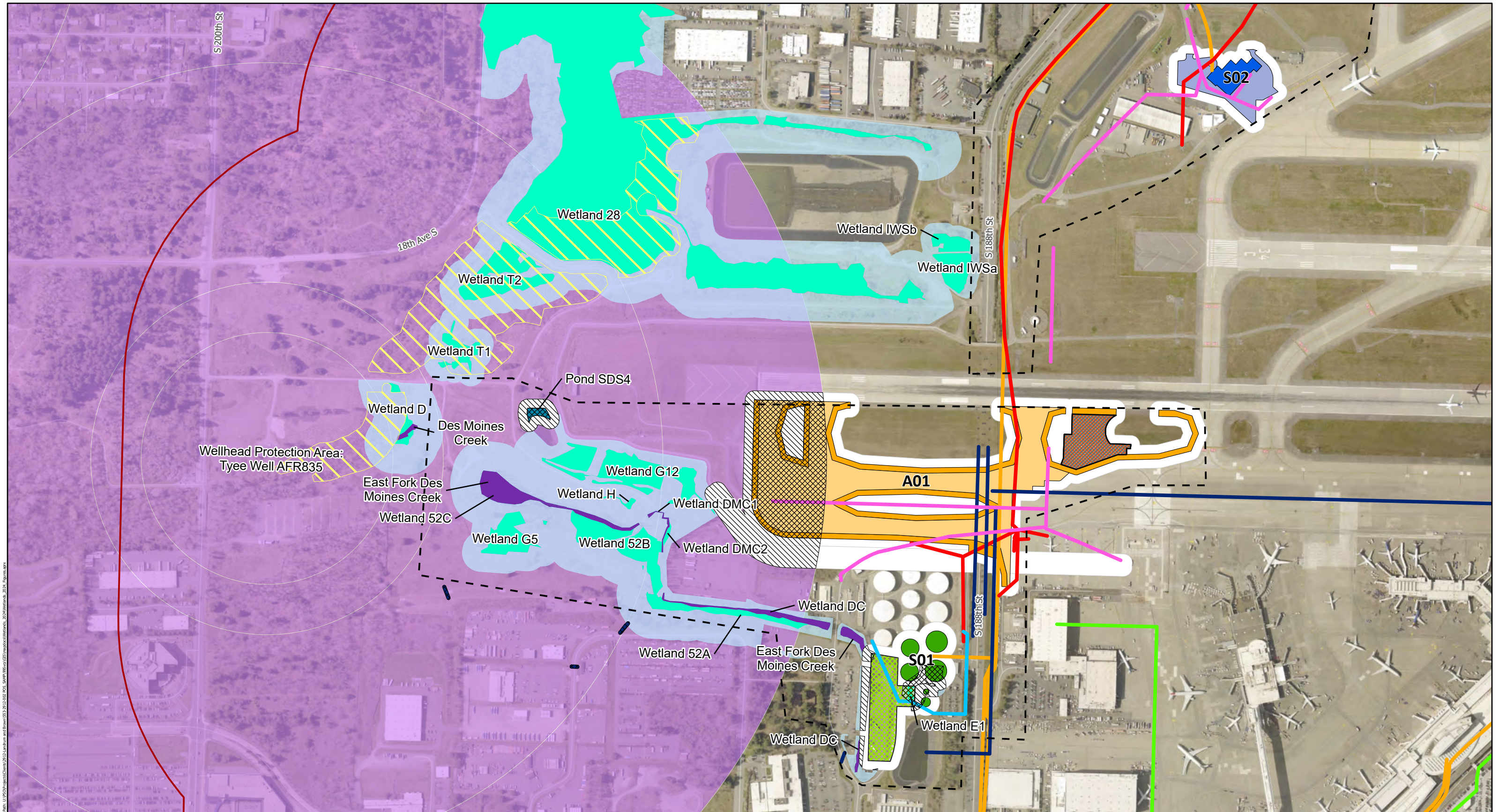
Parametrix Date: 2/12/2024 Sources: King County, King County Aerial (2021) Disclaimer: This product is for informational purposes and may not have been prepared for, or be suitable for legal, engineering, or surveying purposes. Figure 1-6c Project Impacts to Aquatic Critical Areas in North Portion of Survey Area Impact Analysis Memorandum Seattle-Tacoma International Airport Sustainable Airport Master Plan (SAMP) King County, WA
