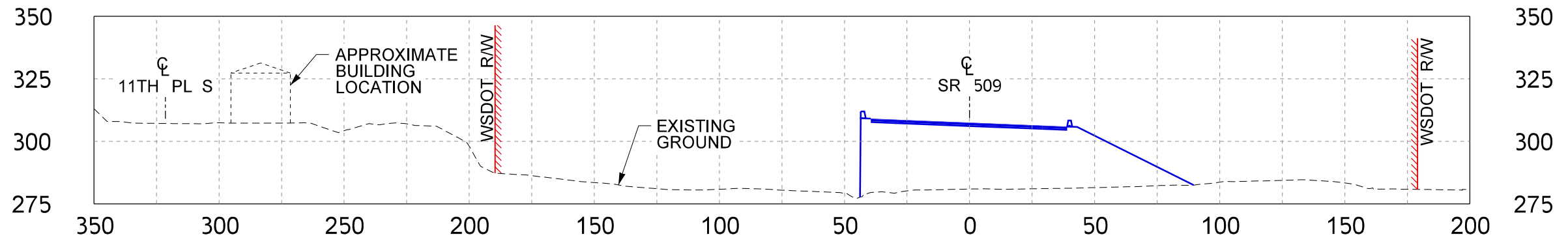
SECTION B-B
