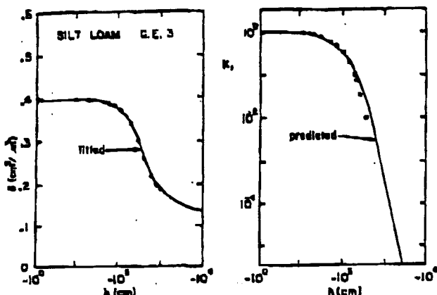
Fig. 7—Observed (open circles) and calculated curves (solid lines) of the soil hydraulic properties of Sils Loam G.E. 3.
