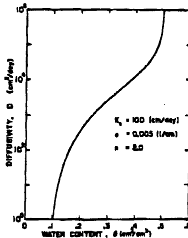
Fig. 2—Plot of the soil-water diffusivity vs. water content as predicted from knowledge of the soil-water retention curve shown in Fig. 1, and the hydraulic conductivity at saturation.
