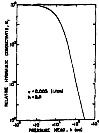
Fig. 3—Plot of the relative hydraulic conductivity vs. pressure head as predicted from knowledge of the soil-water retention curve shown in Fig. 1.
