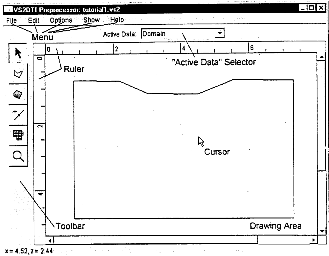
Figure 1. -- Main window of VS2DTI preprocessor.
