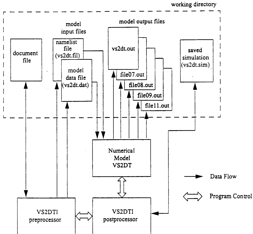
Figure 4. -- Relations between files and preprocessor, postprocessor, and numerical model for VS2DTI.
