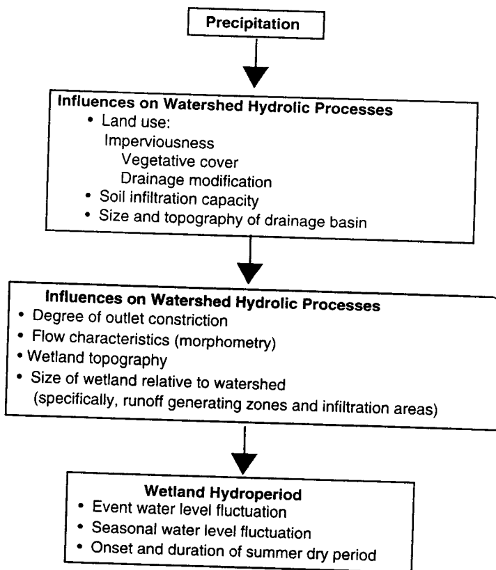
FIGURE 1-3 Conceptual model of influences on wetland hydroperiod.
