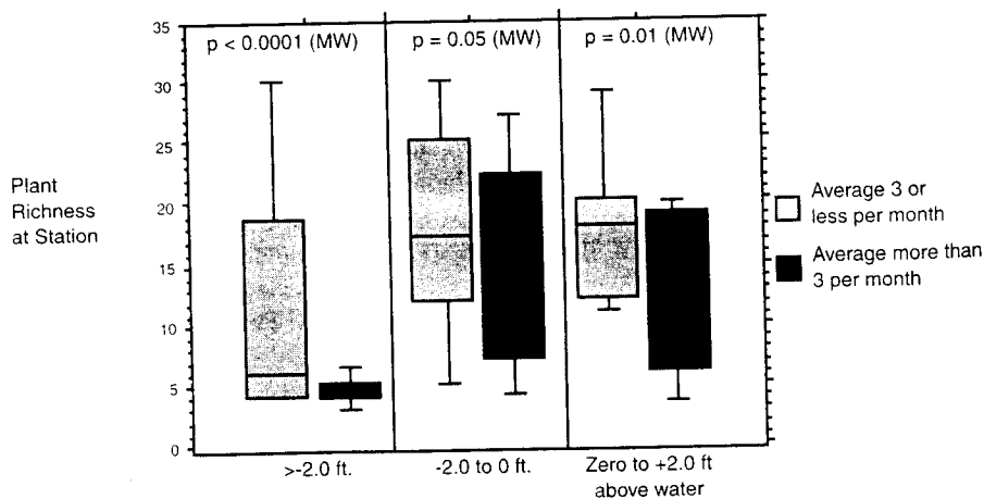
FIGURE 13-1 Plant richness, water depth, and frequency of events.
