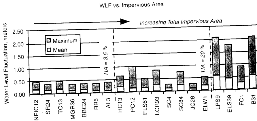
FIGURE 8-2 Relationship between event WLF and impervious area.
