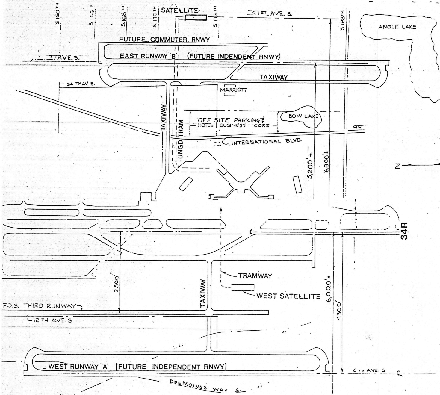
PLAN A FUTURE SEA/TAC AIRPORT EXPANSION WITH AN INDEPENDENT RUNWAY 4300' WEST OF 34R
