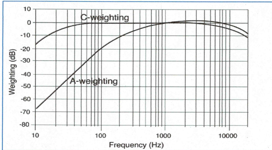
Figure 2. Frequency Response Characteristics of A- and C-Weighting.
