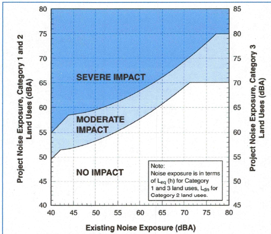
Figure 3. Federal Railroad Administration Noise Metrics/Criteria
