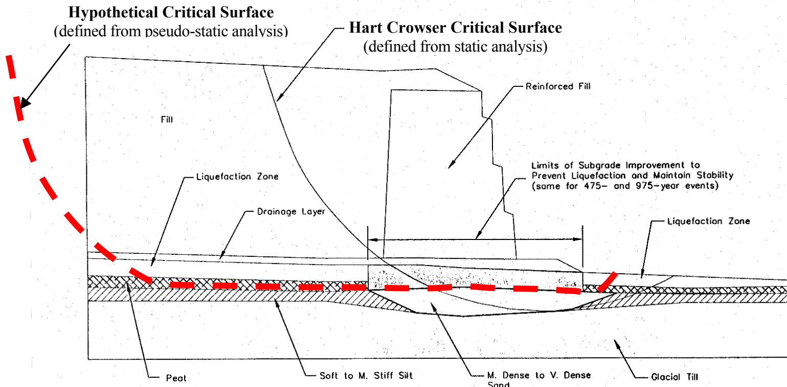
Figure 1: Hypothetical Seismic Stability Failure Surface
