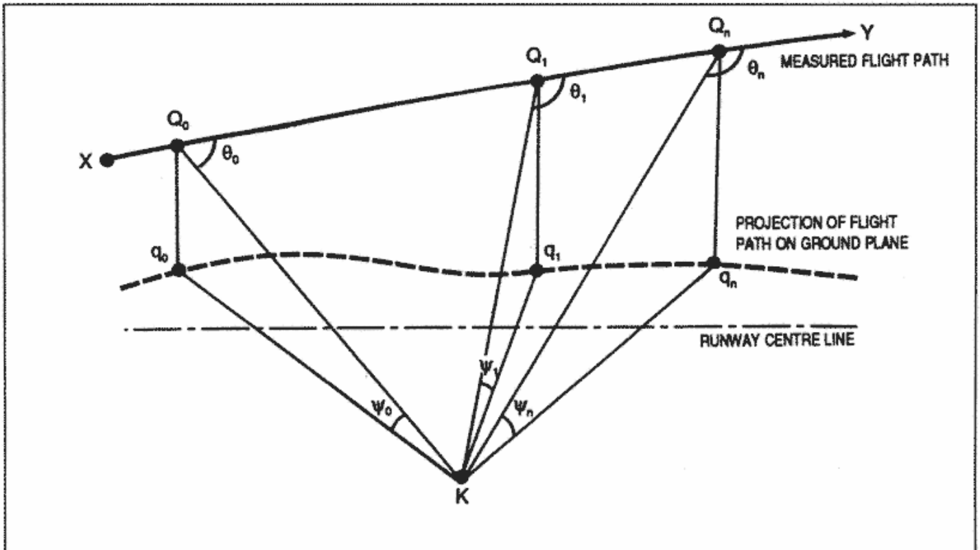
Figure A36-11(a). Measured flight path
