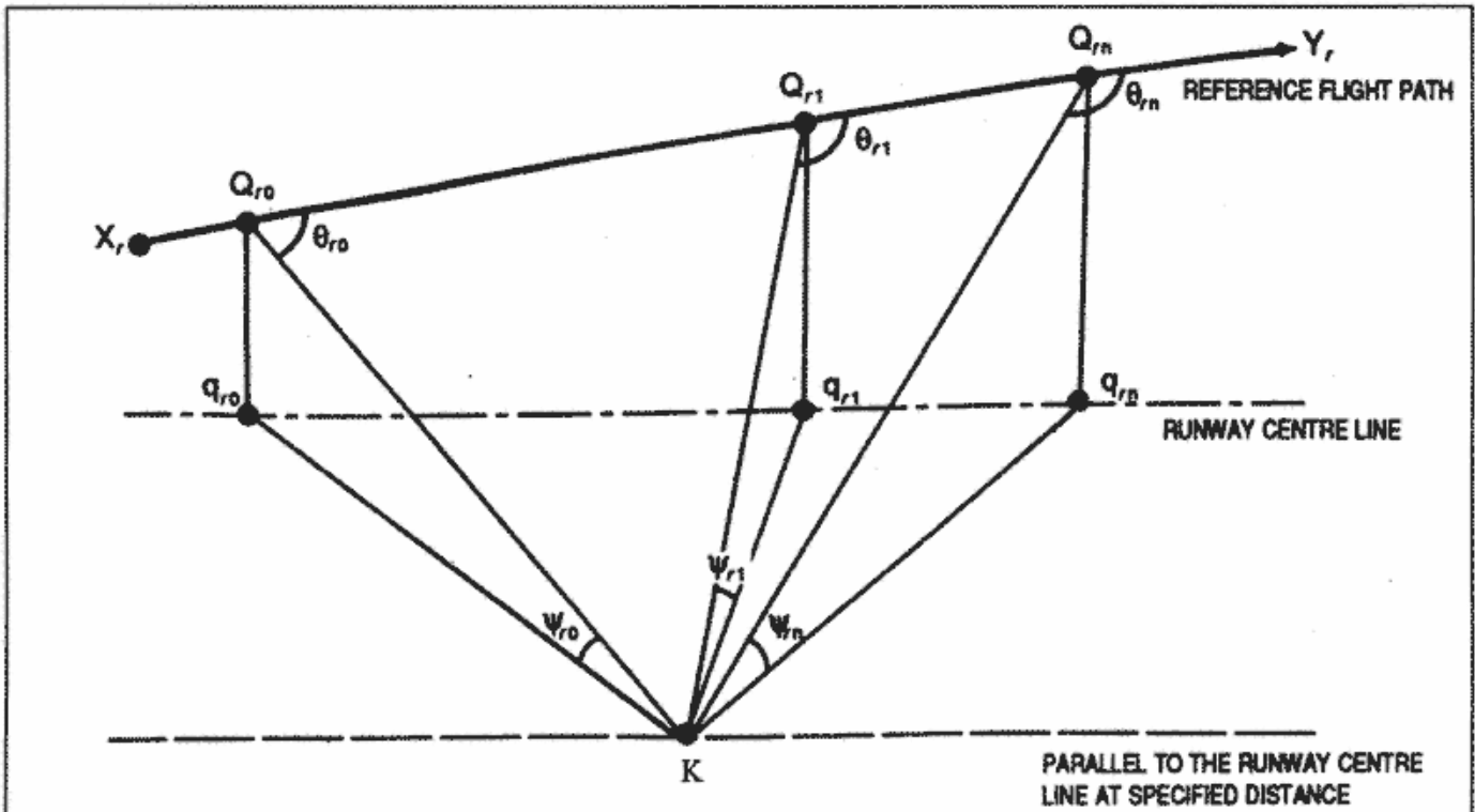
Figure A36-11(b). Reference flight path
