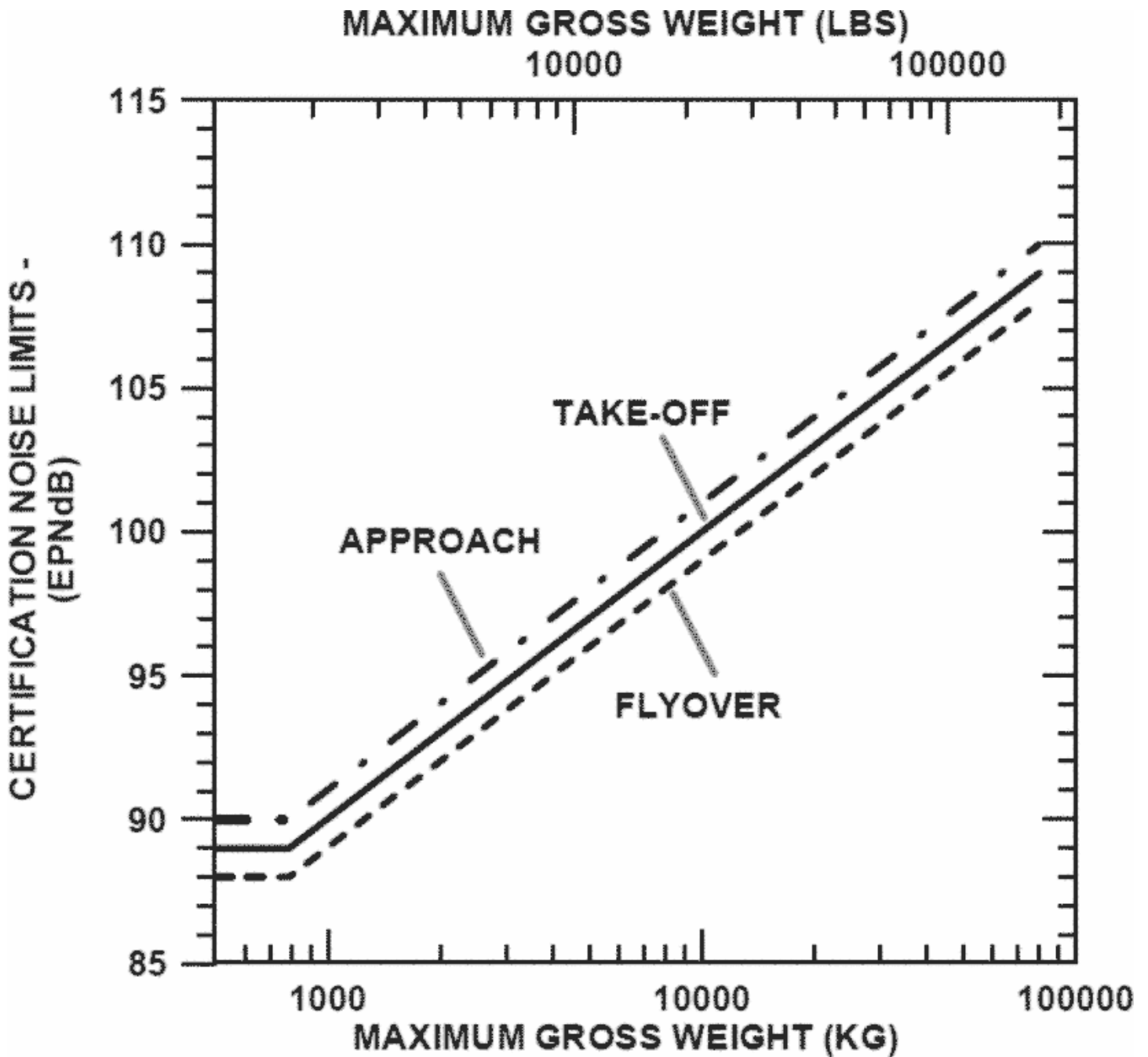
FIGURE K4. TILTROTOR NOISE LIMITS
